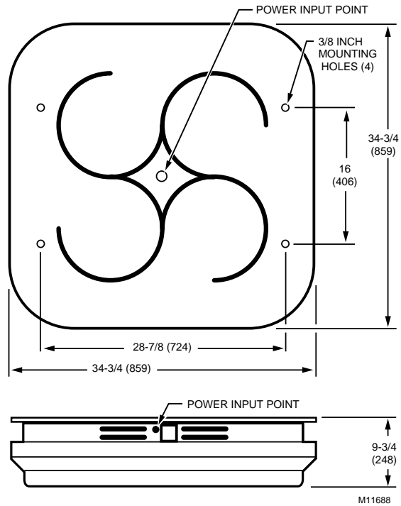
Fig 1. F115 dimensions in in. (mm).
